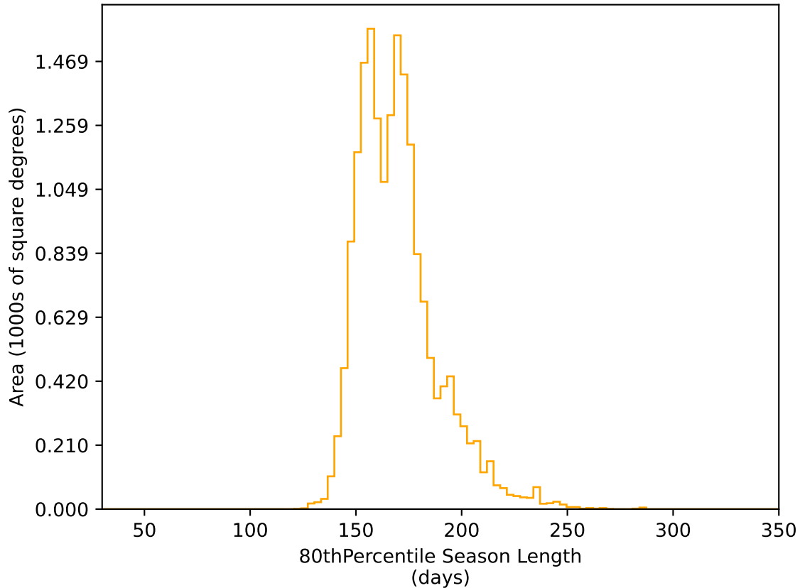
ddf_acor_sf15_lsf40_lsr50_v3.4_10yrs WFD r band: 80thPercentile Season Length
