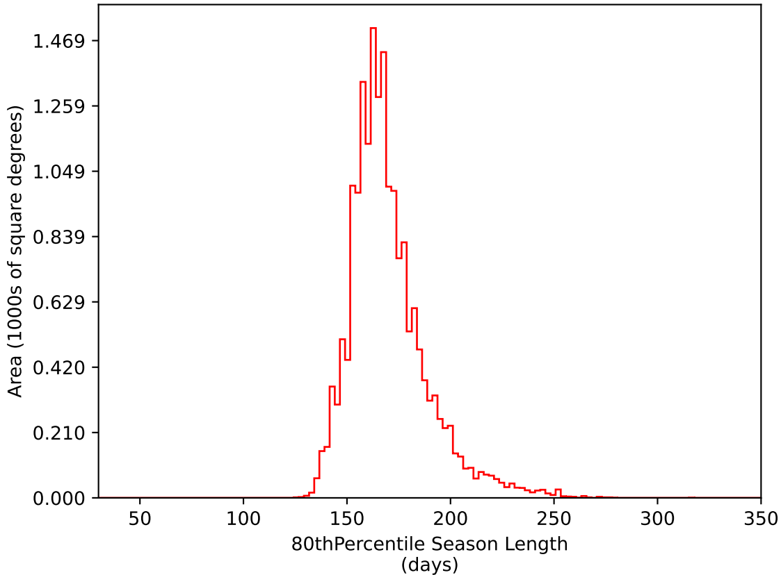
ddf_acor_sf15_lsf40_lsr50_v3.4_10yrs WFD i band: 80thPercentile Season Length
