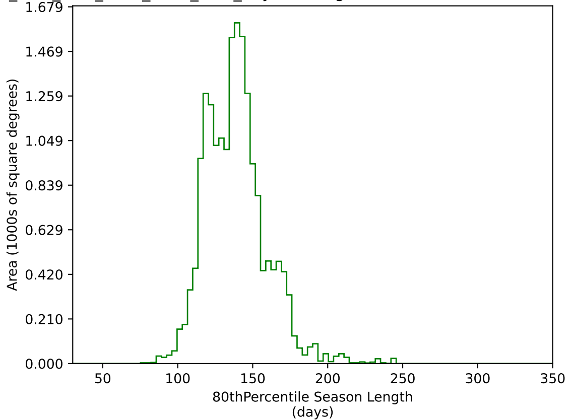
ddf_acor_sf15_lsf40_lsr50_v3.4_10yrs WFD g band: 80thPercentile Season Length
