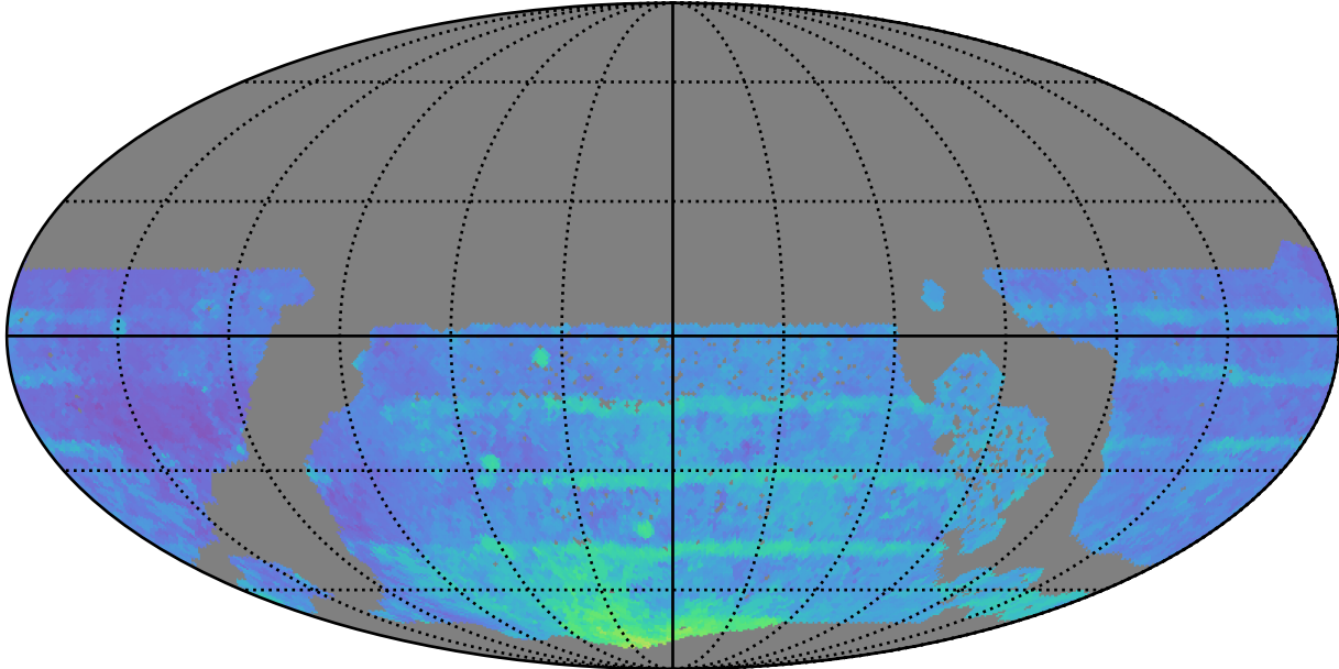
ddf_acor_sf15_lsf40_lsr50_v3.4_10yrs WFD all bands: 80thPercentile Season Length
