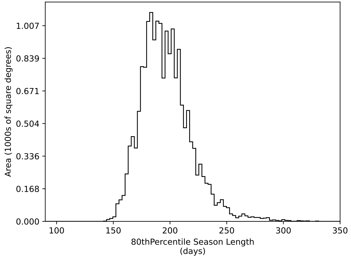
ddf_acor_sf15_lsf40_lsr50_v3.4_10yrs WFD all bands: 80thPercentile Season Length
