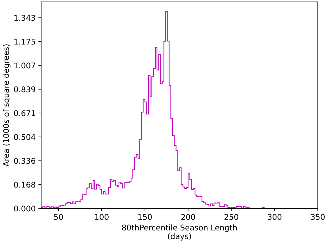
ddf_acor_sf15_lsf40_lsr50_v3.4_10yrs All sky z band: 80thPercentile Season Length
