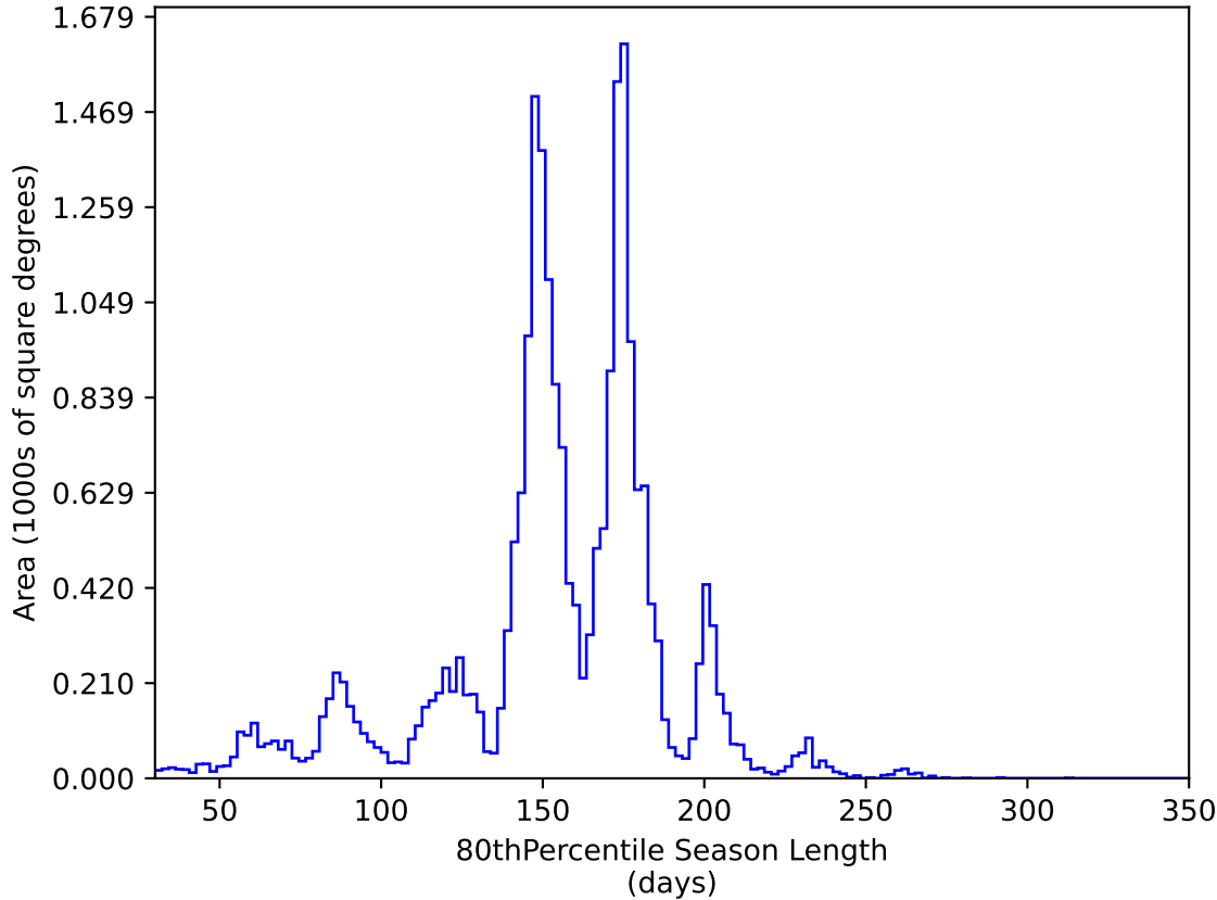
ddf_acor_sf15_lsf40_lsr50_v3.4_10yrs All sky y band: 80thPercentile Season Length
