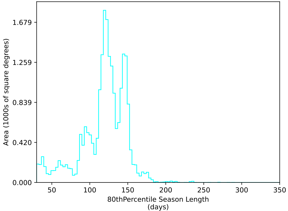
ddf_acor_sf15_lsf40_lsr50_v3.4_10yrs All sky u band: 80thPercentile Season Length
