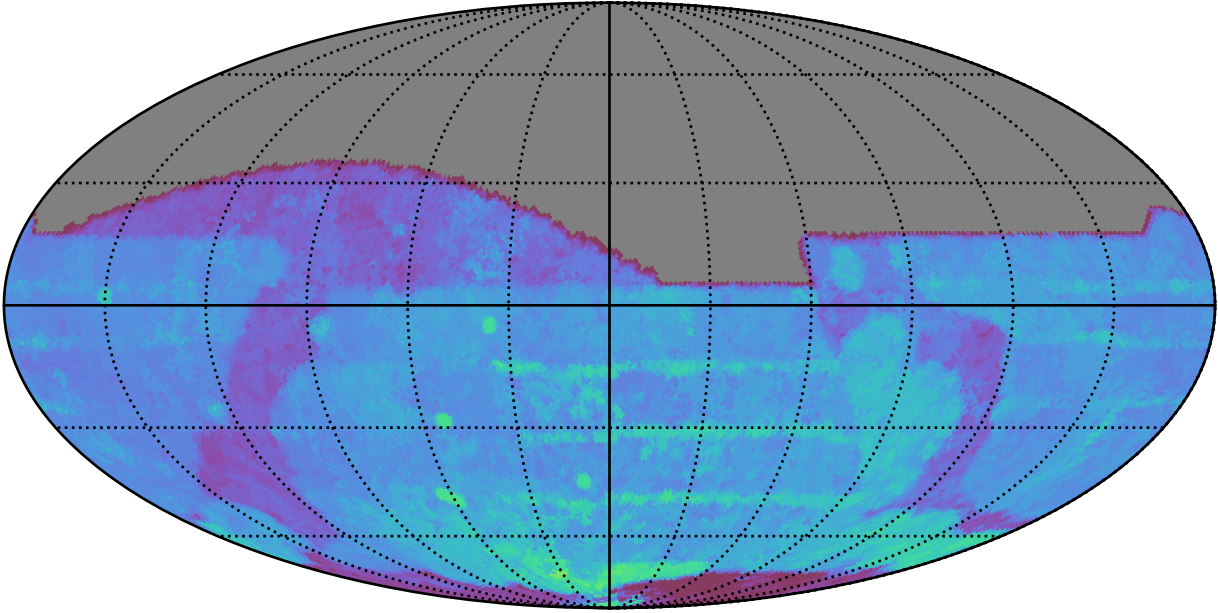
ddf_acor_sf15_lsf40_lsr50_v3.4_10yrs All sky r band: 80thPercentile Season Length
