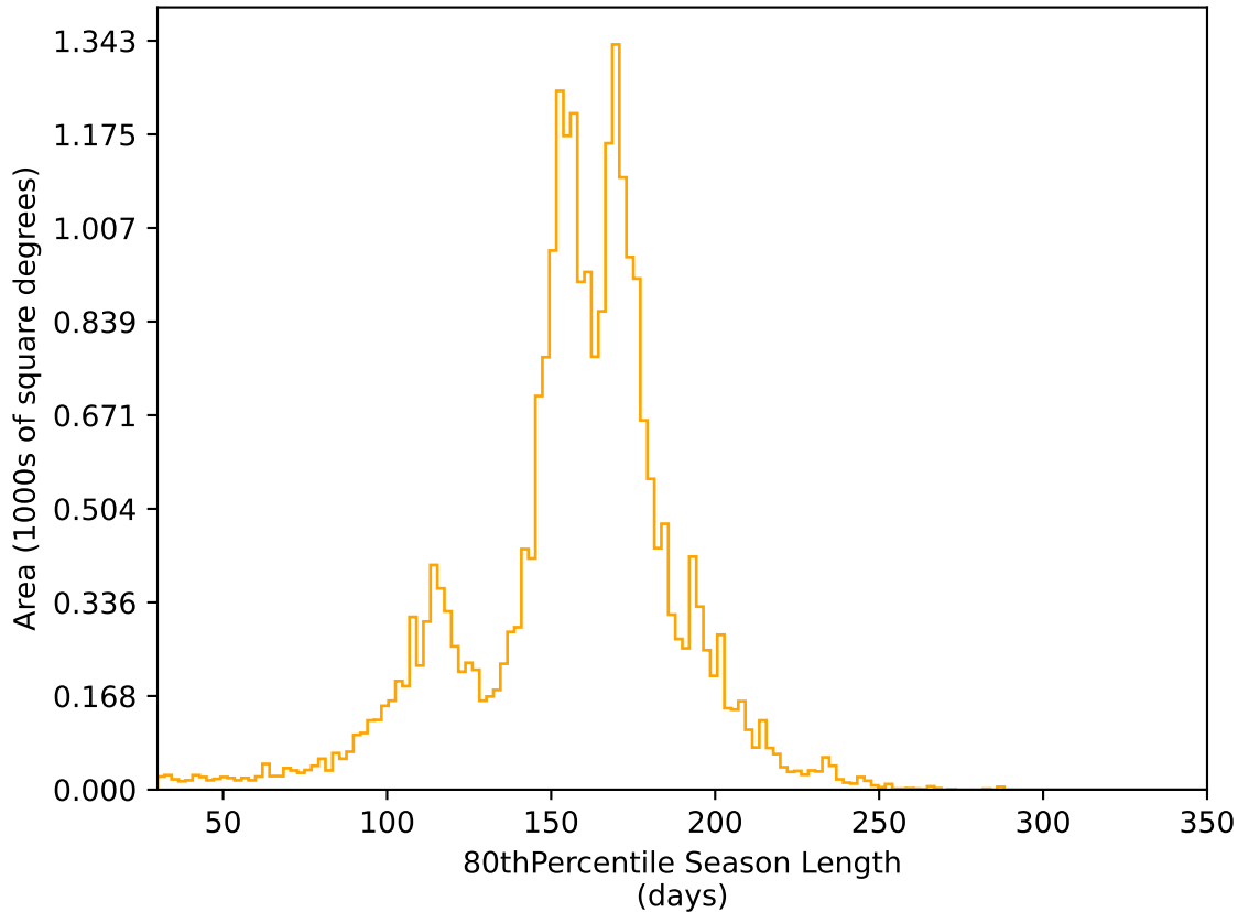
ddf_acor_sf15_lsf40_lsr50_v3.4_10yrs All sky r band: 80thPercentile Season Length
