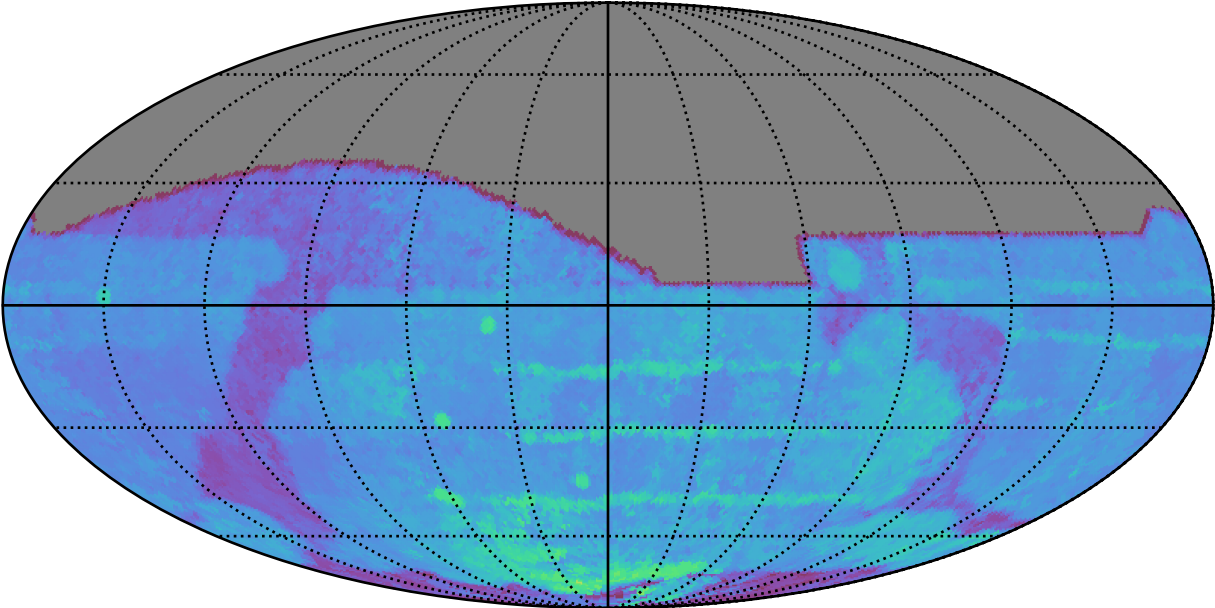
ddf_acor_sf15_lsf40_lsr50_v3.4_10yrs All sky i band: 80thPercentile Season Length
