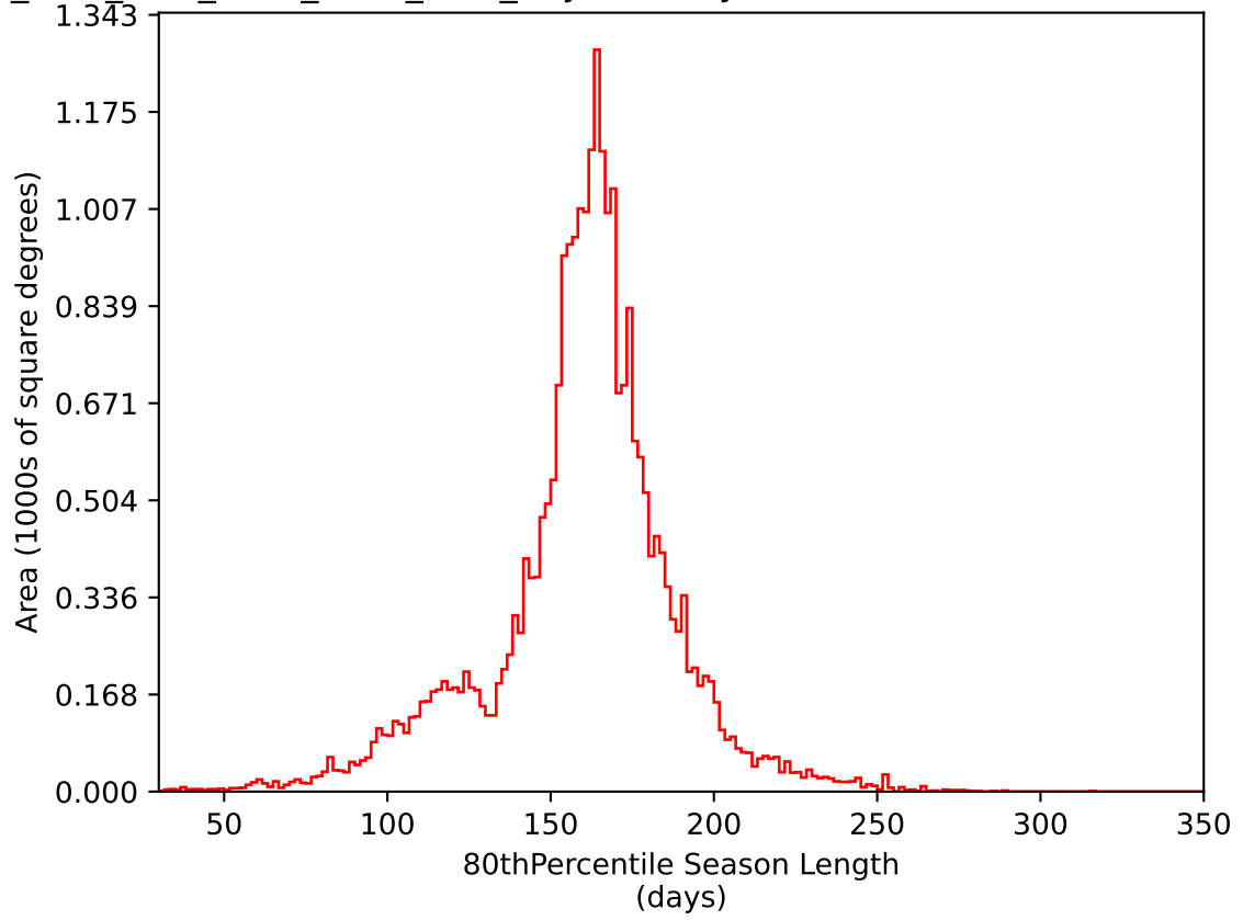
ddf_acor_sf15_lsf40_lsr50_v3.4_10yrs All sky i band: 80thPercentile Season Length
