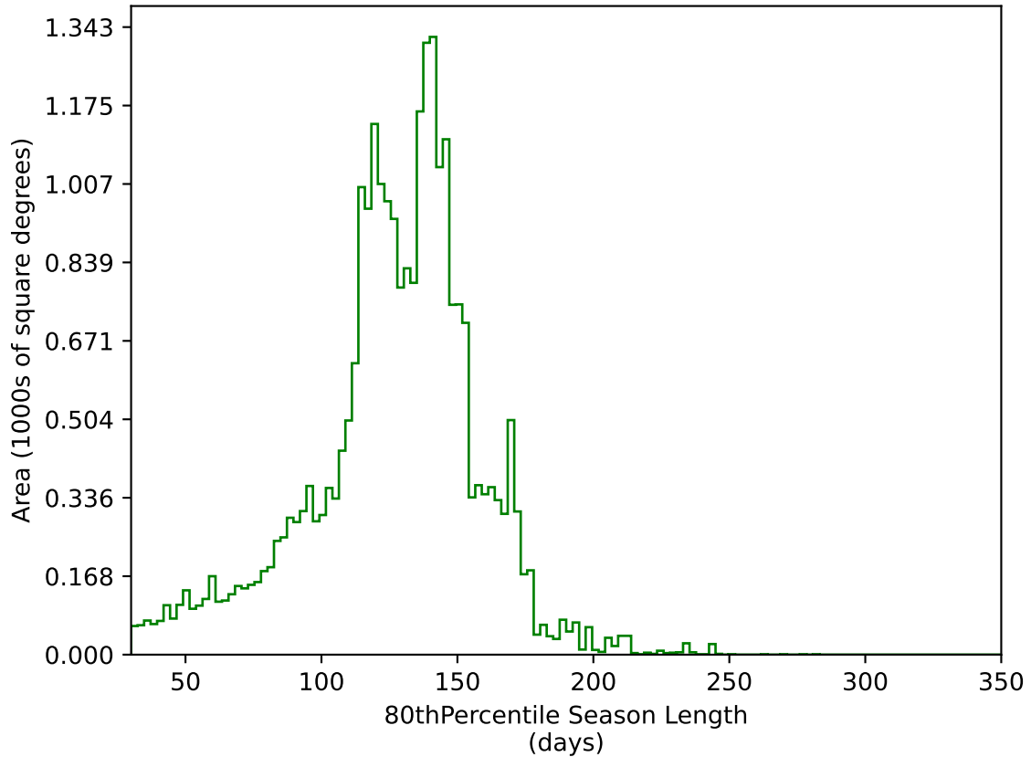
ddf_acor_sf15_ls40_lsr50_v3.4_10yrs All sky g band: 80thPercentile Season Length
