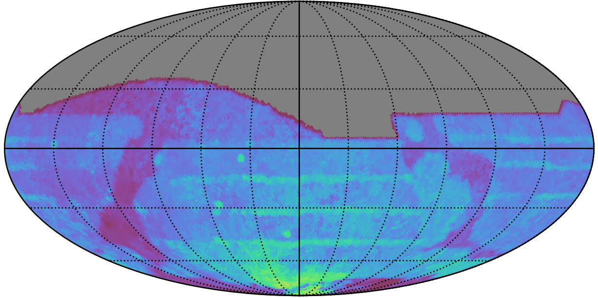
ddf_acor_sf15_lsf40_lsr50_v3.4_10yrs All sky all bands: 80thPercentile Season Length
