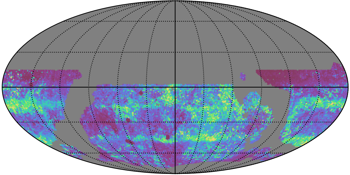
ddf_acor_sf15_lsf40_lsr50_v3.4_10yrs WFD zy bands: 75th Percentile Intranight Timespan
