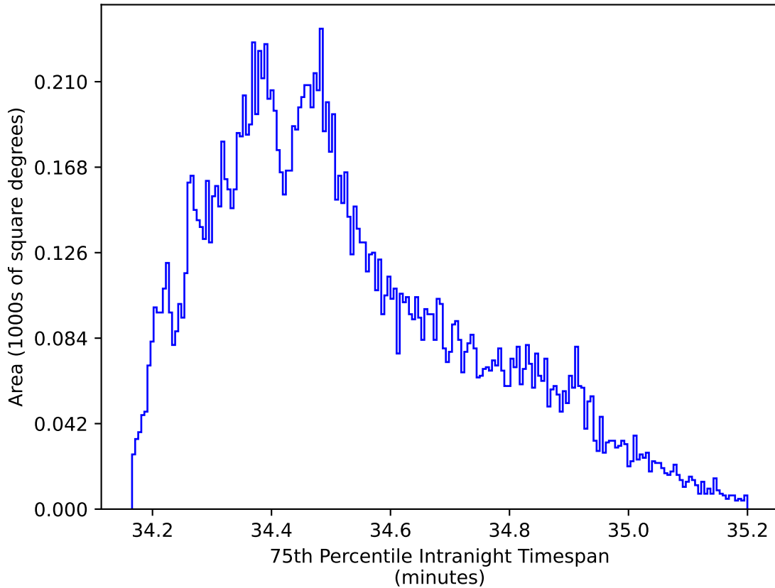
ddf_acor_sf15_lsf40_lsr50_v3.4_10yrs WFD zy bands: 75th Percentile Intranight Timespan
