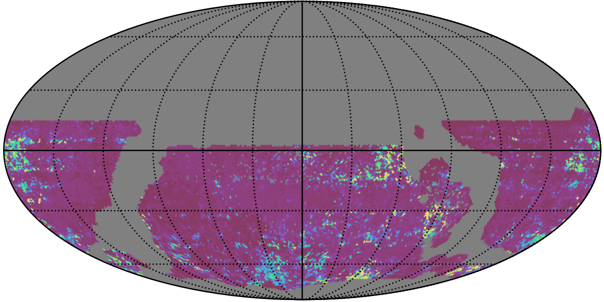
ddf_acor_sf15_lsf40_lsr50_v3.4_10yrs WFD z band: 75th Percentile Intranight Timespan
