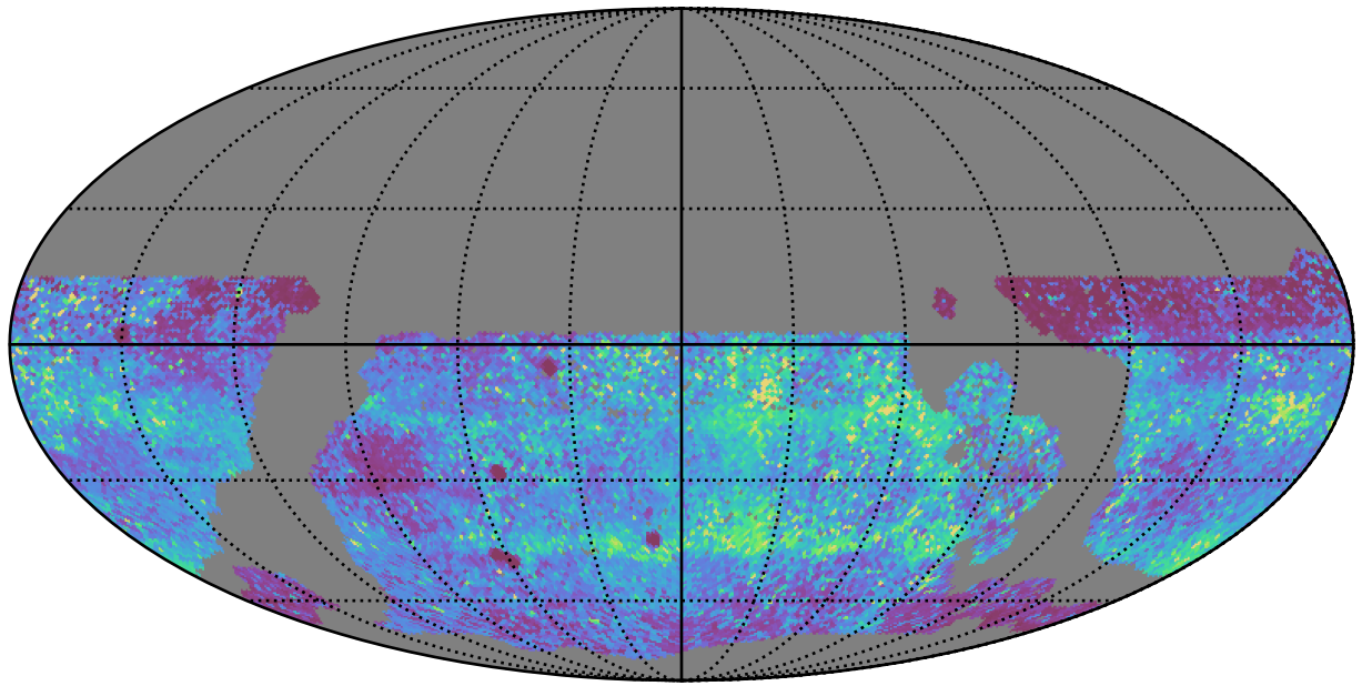
ddf_acor_sf15_lsf40_lsr50_v3.4_10yrs WFD y band: 75th Percentile Intranight Timespan
