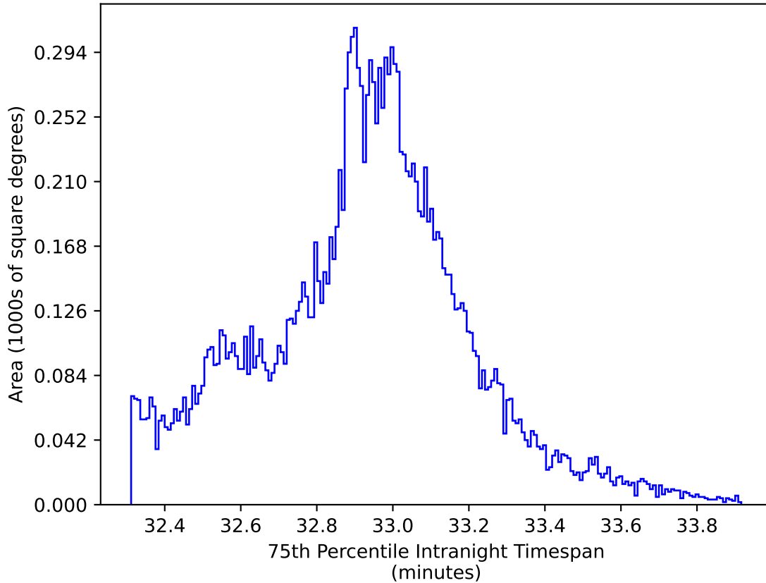
ddf_acor_sf15_lsf40_lsr50_v3.4_10yrs WFD y band: 75th Percentile Intranight Timespan
