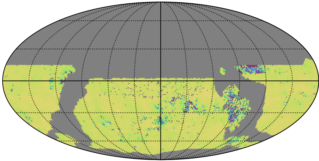
ddf_acor_sf15_lsf40_lsr50_v3.4_10yrs WFD ug bands: 75th Percentile Intranight Timespan
