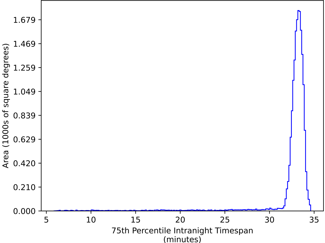
ddf_acor_sf15_lsf40_lsr50_v3.4_10yrs WFD ug bands: 75th Percentile Intranight Timespan
