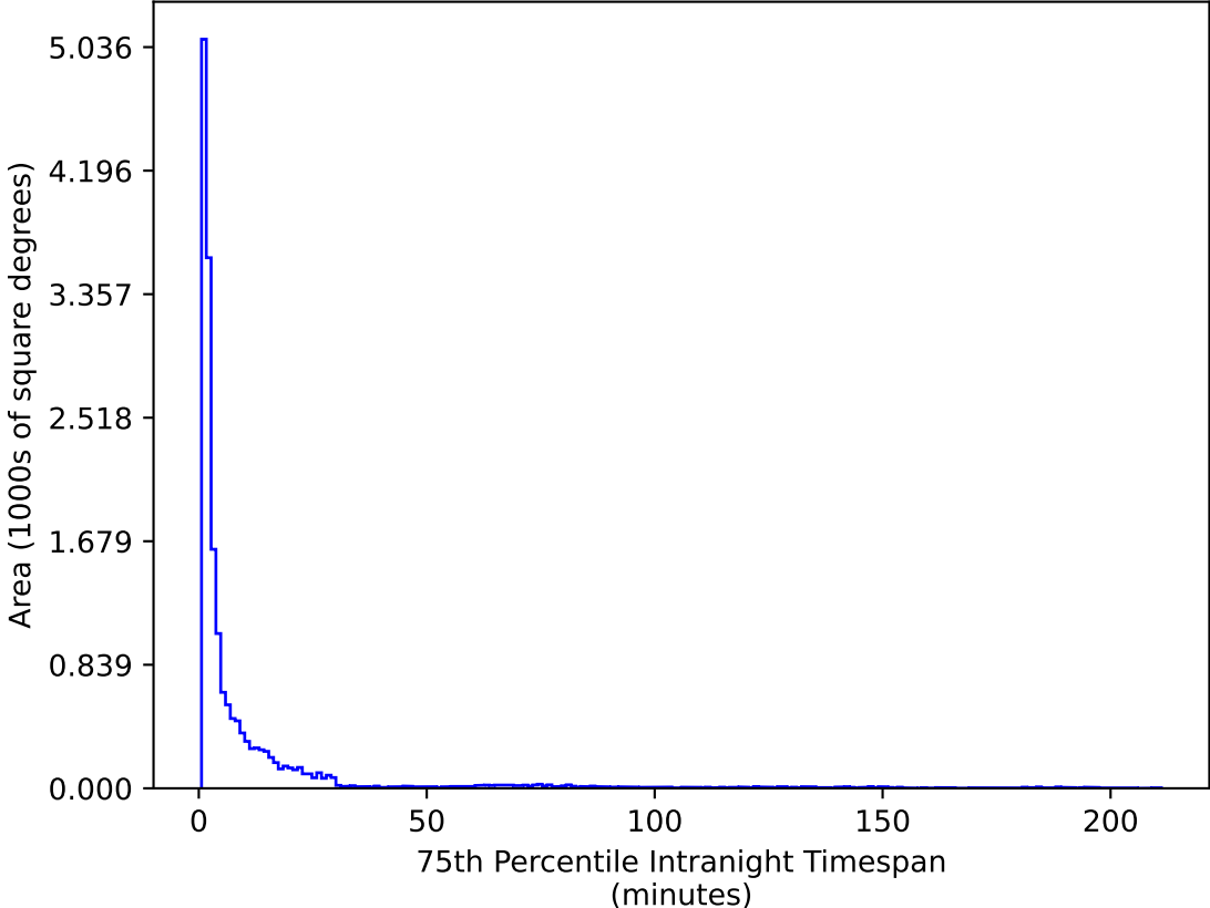
ddf_acor_sf15_lsf40_lsr50_v3.4_10yrs WFD u band: 75th Percentile Intranight Timespan
