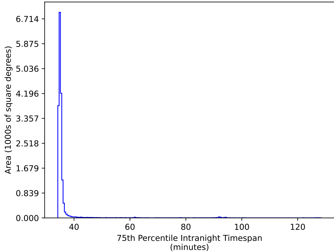
ddf_acor_sf15_lsf40_lsr50_v3.4_10yrs WFD ri bands: 75th Percentile Intranight Timespan
