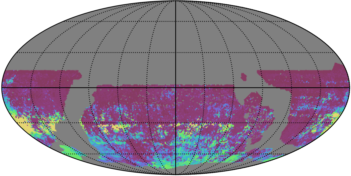
ddf_acor_sf15_lsf40_lsr50_v3.4_10yrs WFD r band: 75th Percentile Intranight Timespan
