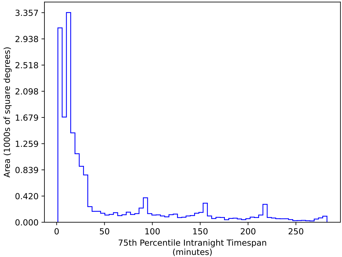
ddf_acor_sf15_lsf40_lsr50_v3.4_10yrs WFD r band: 75th Percentile Intranight Timespan
