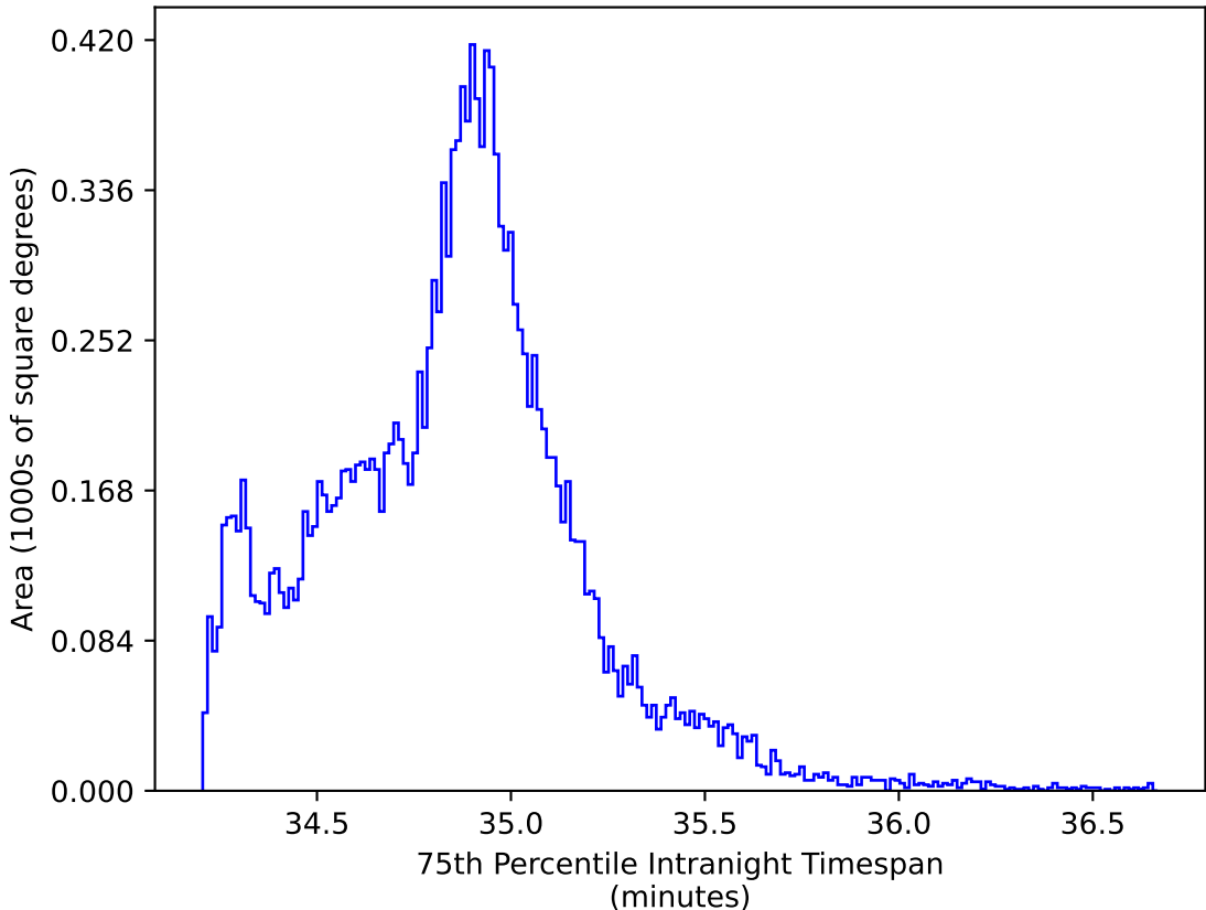
ddf_acor_sf15_lsf40_lsr50_v3.4_10yrs WFD iz bands: 75th Percentile Intranight Timespan
