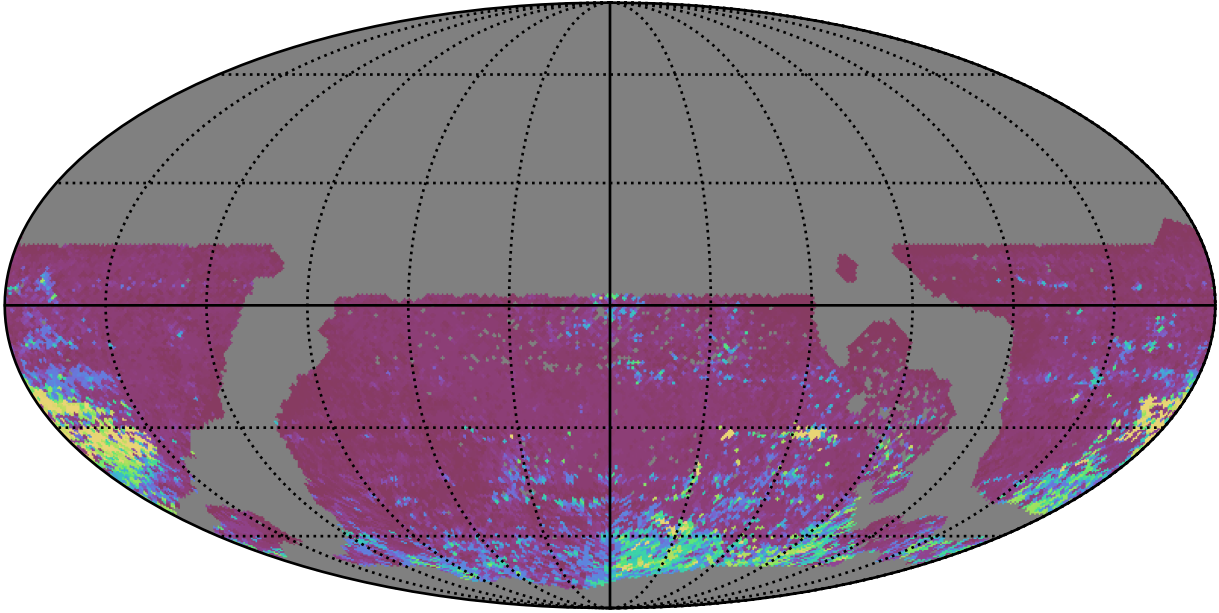
ddf_acor_sf15_lsf40_lsr50_v3.4_10yrs WFD i band: 75th Percentile Intranight Timespan
