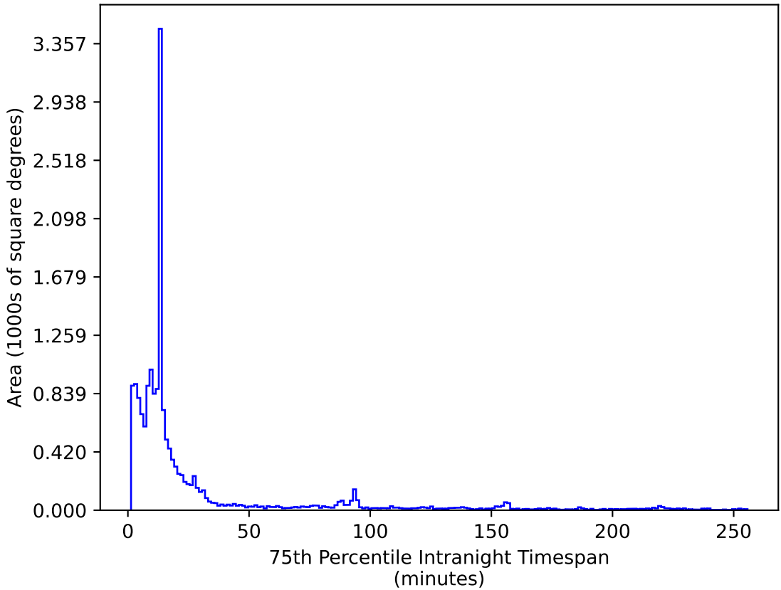
ddf_acor_sf15_lsf40_lsr50_v3.4_10yrs WFD i band: 75th Percentile Intranight Timespan
