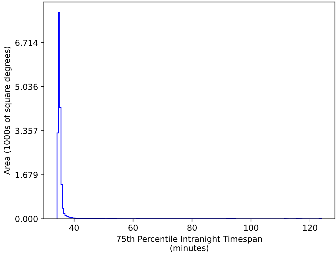
ddf_acor_sf15_lsf40_lsr50_v3.4_10yrs WFD gr bands: 75th Percentile Intranight Timespan
