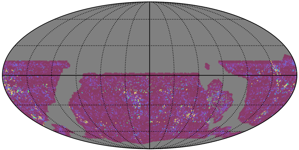
ddf_acor_sf15_lsf40_lsr50_v3.4_10yrs WFD g band: 75th Percentile Intranight Timespan
