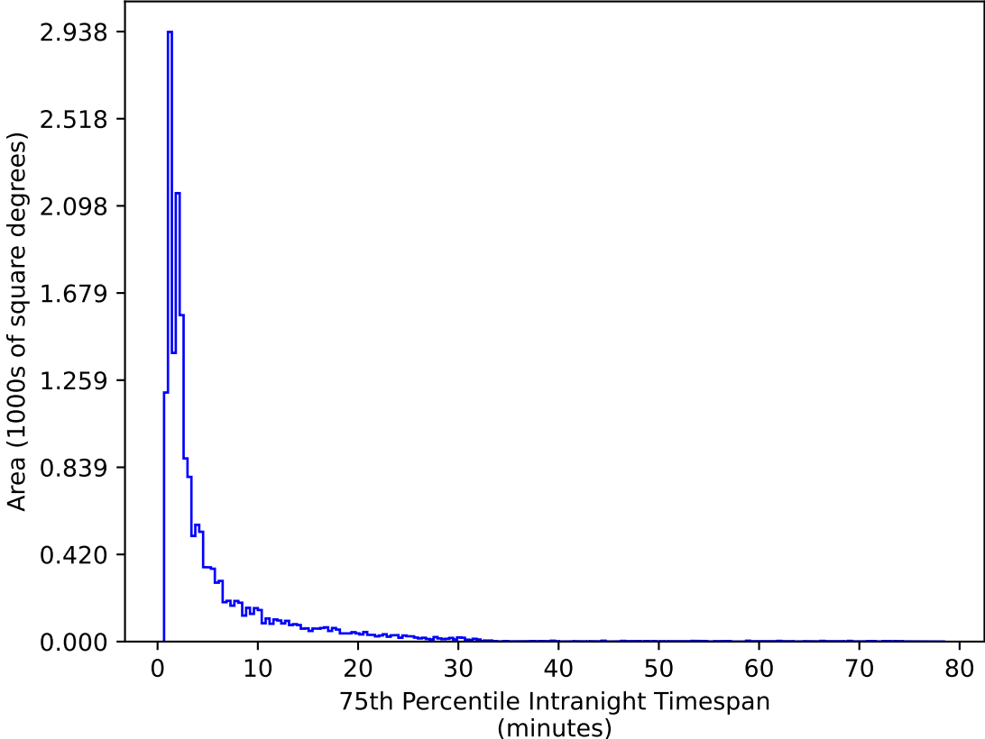
ddf_acor_sf15_lsf40_lsr50_v3.4_10yrs WFD g band: 75th Percentile Intranight Timespan
