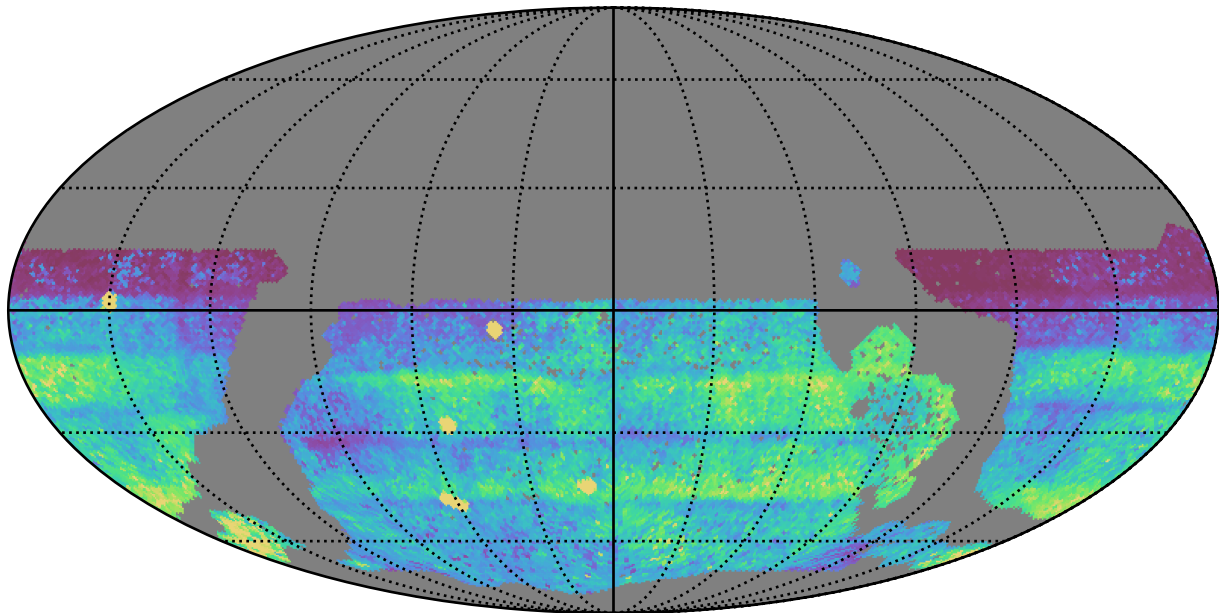
ddf_acor_sf15_lsf40_lsr50_v3.4_10yrs WFD all bands: 75th Percentile Intranight Timespan
