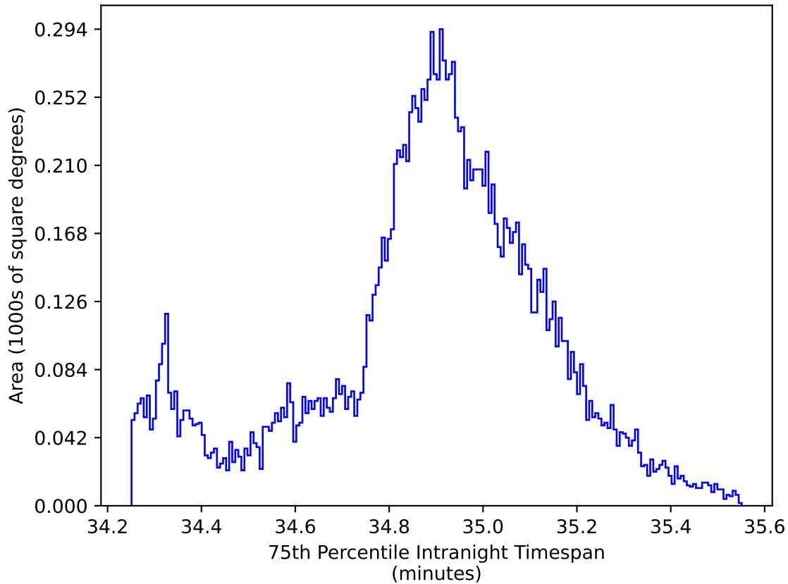
ddf_acor_sf15_lsf40_lsr50_v3.4_10yrs WFD all bands: 75th Percentile Intranight Timespan
