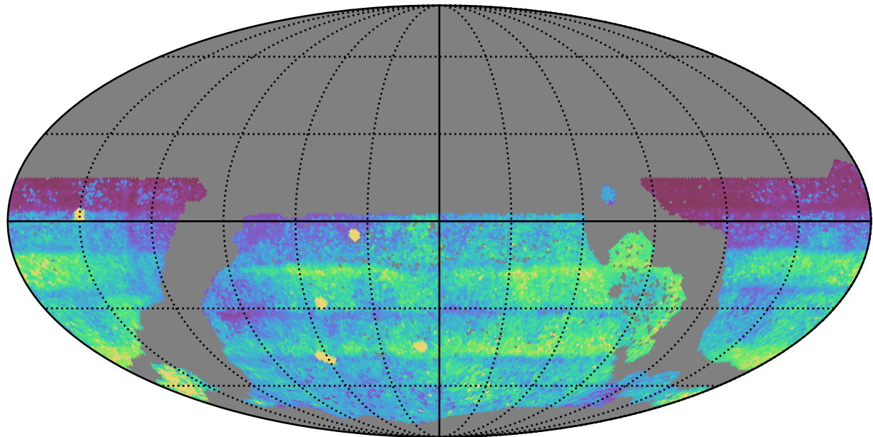
ddf_acor_sf15_lsf40_lsr50_v3.4_10yrs WFD: 75th Percentile Intranight Timespan
