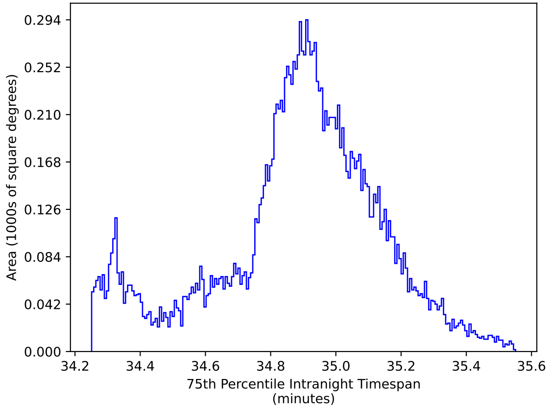
ddf_acor_sf15_ls40_lsr50_v3.4_10yrs WFD: 75th Percentile Intranight Timespan
