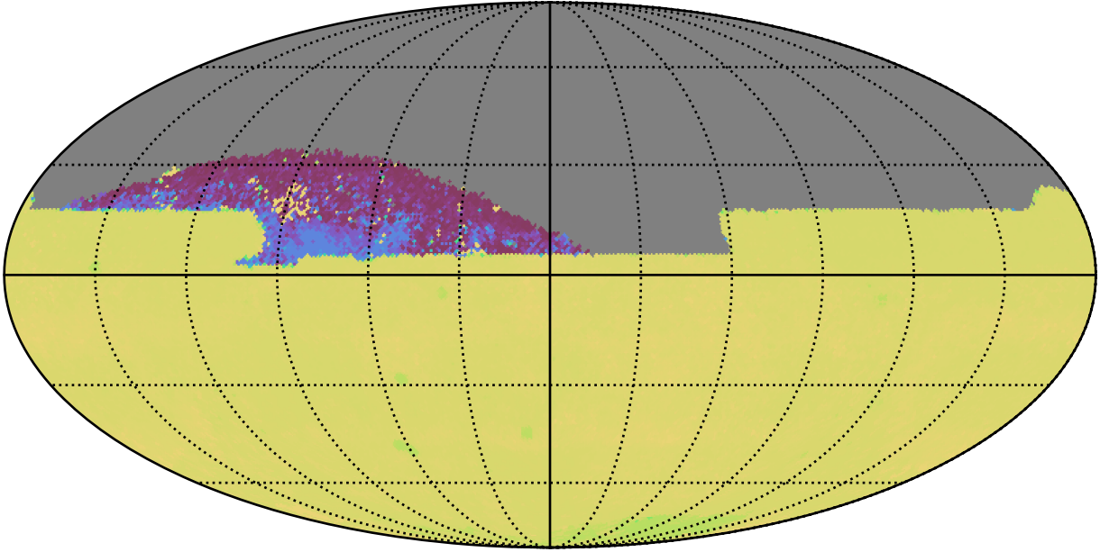
ddf_acor_sf15_lsf40_lsr50_v3.4_10yrs All sky zy bands: 75th Percentile Intranight Timespan
