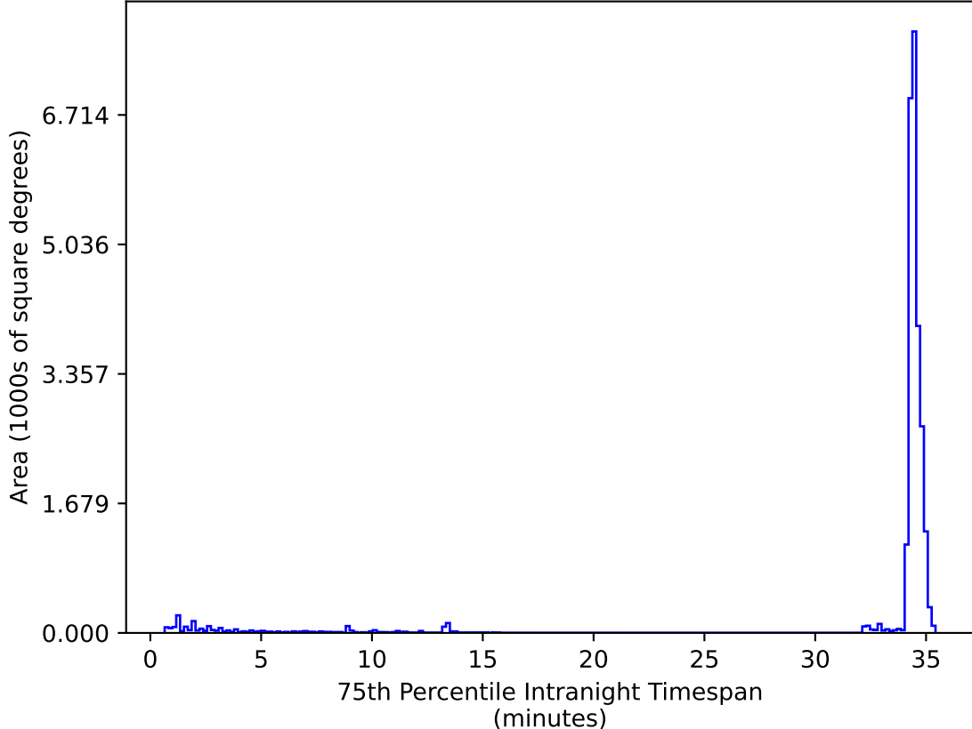
ddf_acor_sf15_lsf40_lsr50_v3.4_10yrs All sky zy bands: 75th Percentile Intranight Timespan
