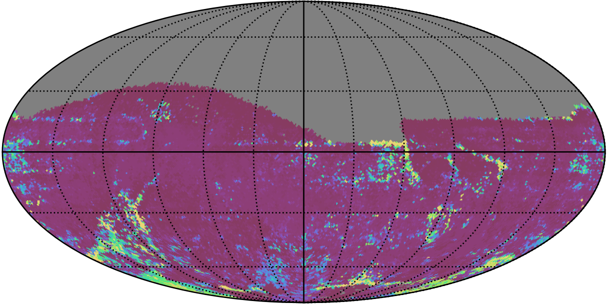
ddf_acor_sf15_lsf40_lsr50_v3.4_10yrs All sky z band: 75th Percentile Intranight Timespan
