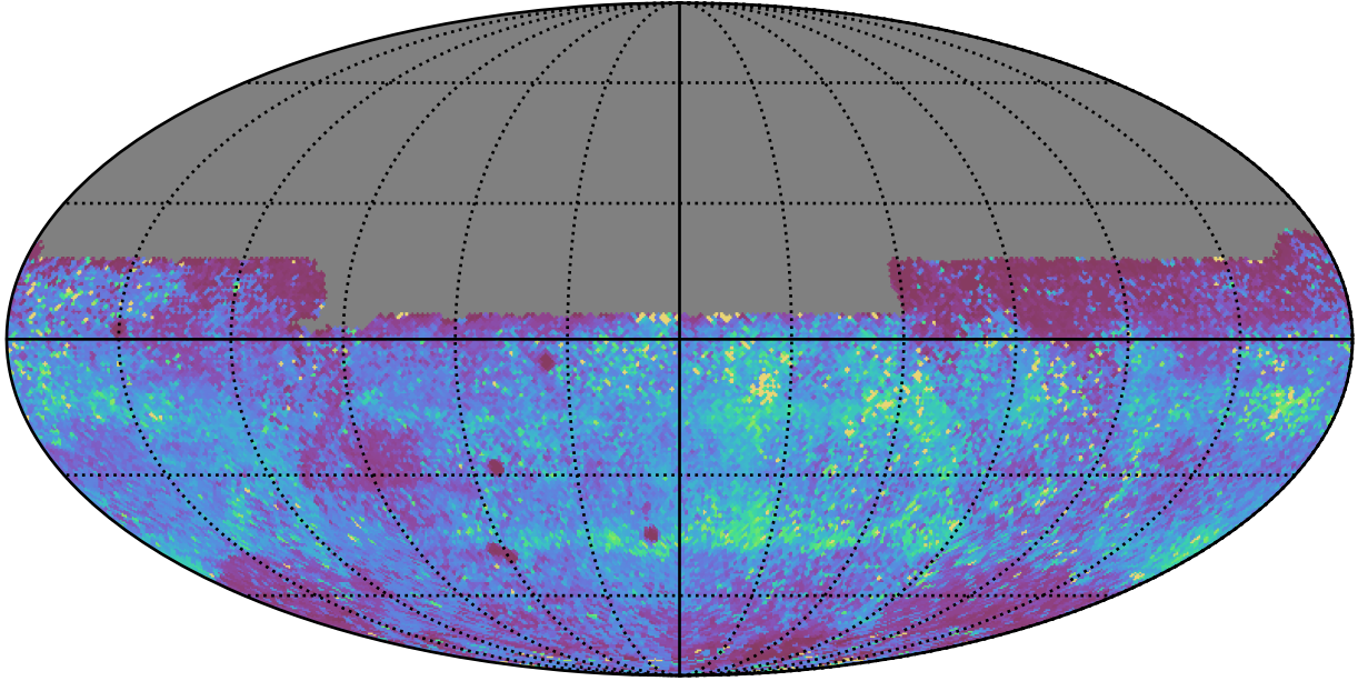
ddf_acor_sf15_lsf40_lsr50_v3.4_10yrs All sky y band: 75th Percentile Intranight Timespan
