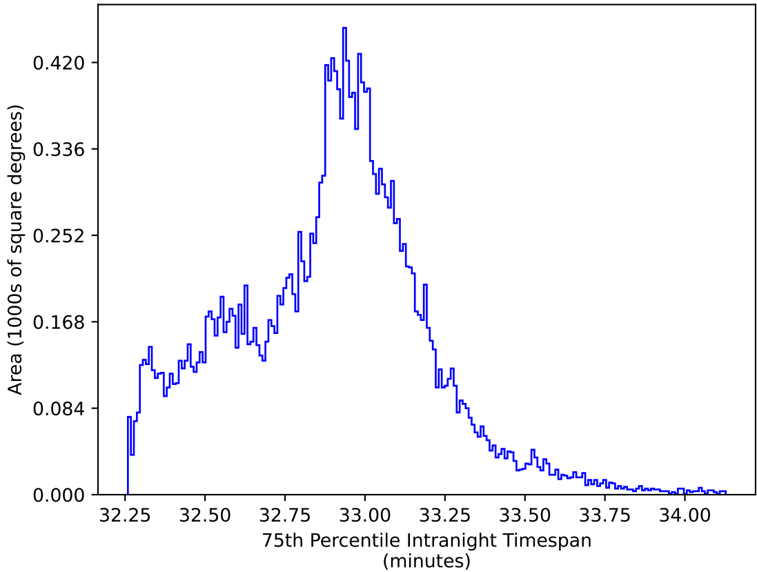
ddf_acor_sf15_lsf40_lsr50_v3.4_10yrs All sky y band: 75th Percentile Intranight Timespan
