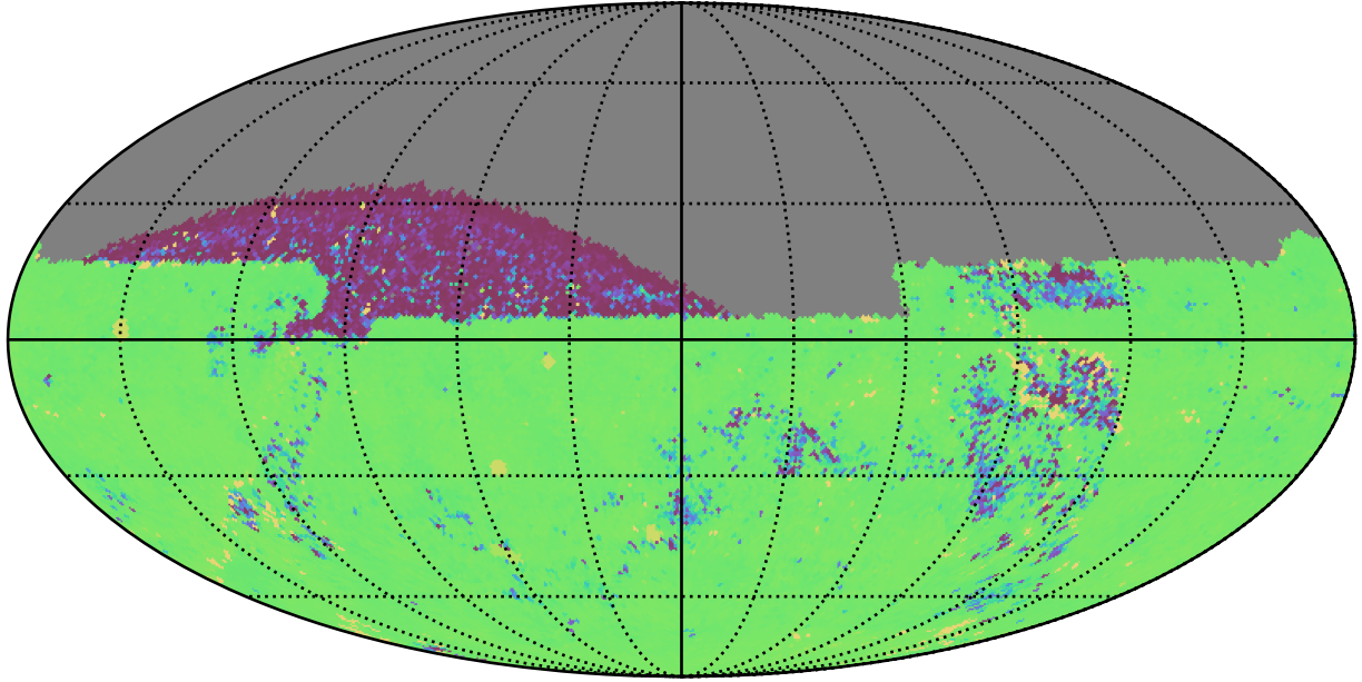
ddf_acor_sf15_lsf40_lsr50_v3.4_10yrs All sky ug bands: 75th Percentile Intranight Timespan
