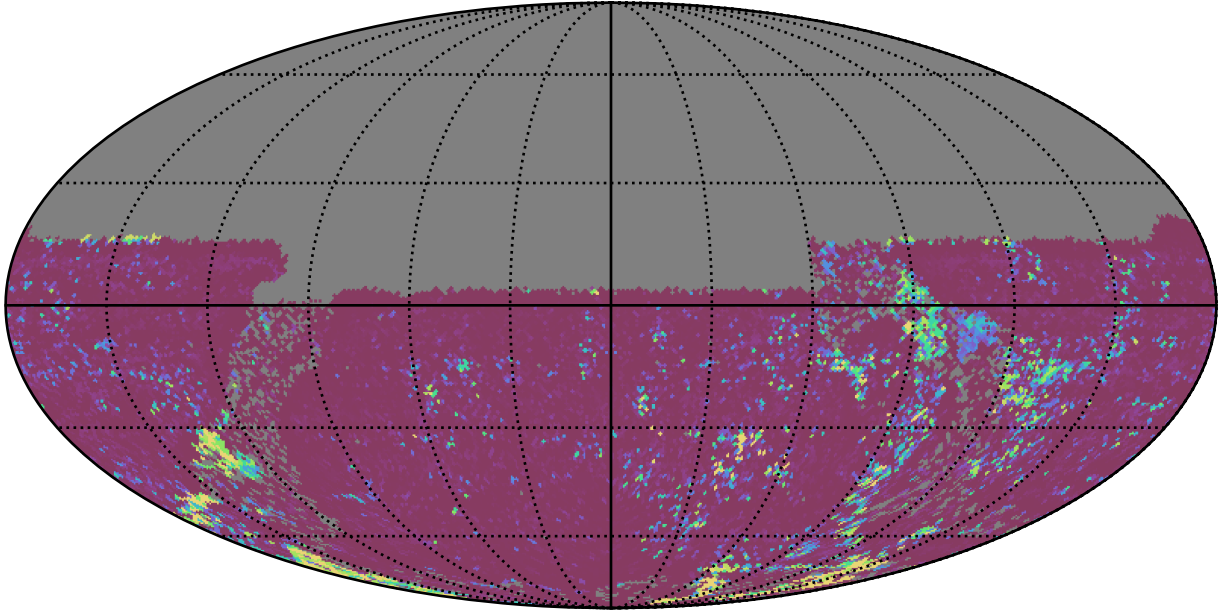
ddf_acor_sf15_lsf40_lsr50_v3.4_10yrs All sky u band: 75th Percentile Intranight Timespan
