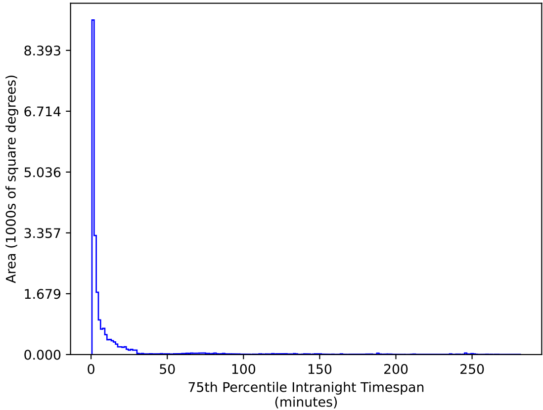
ddf_acor_sf15_lsf40_lsr50_v3.4_10yrs All sky u band: 75th Percentile Intranight Timespan
