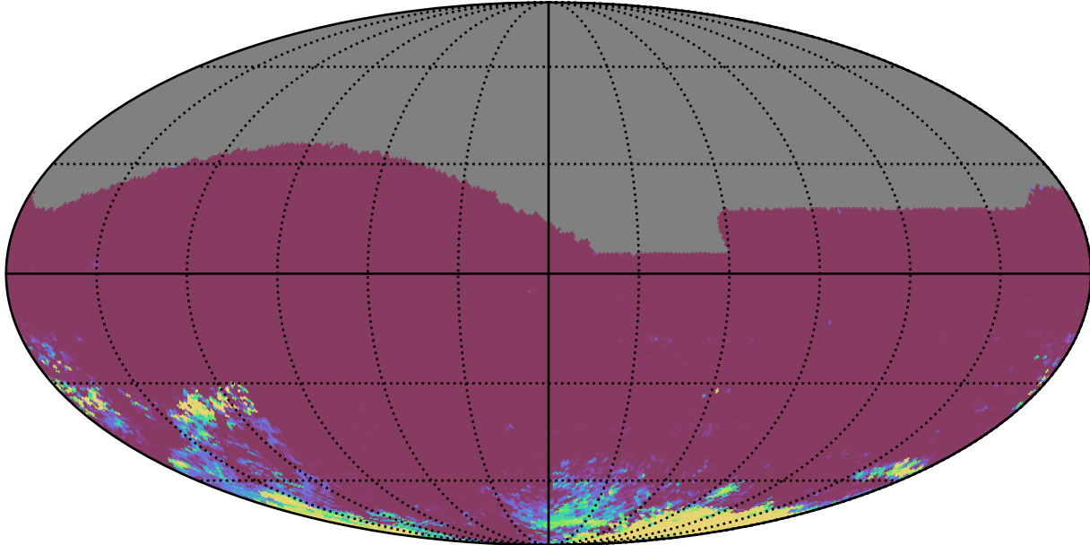
ddf_acor_sf15_lsf40_lsr50_v3.4_10yrs All sky ri bands: 75th Percentile Intranight Timespan
