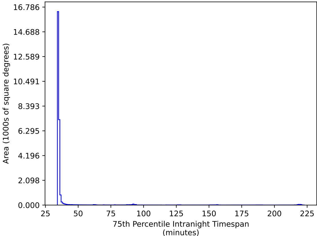
ddf_acor_sf15_lsf40_lsr50_v3.4_10yrs All sky ri bands: 75th Percentile Intranight Timespan
