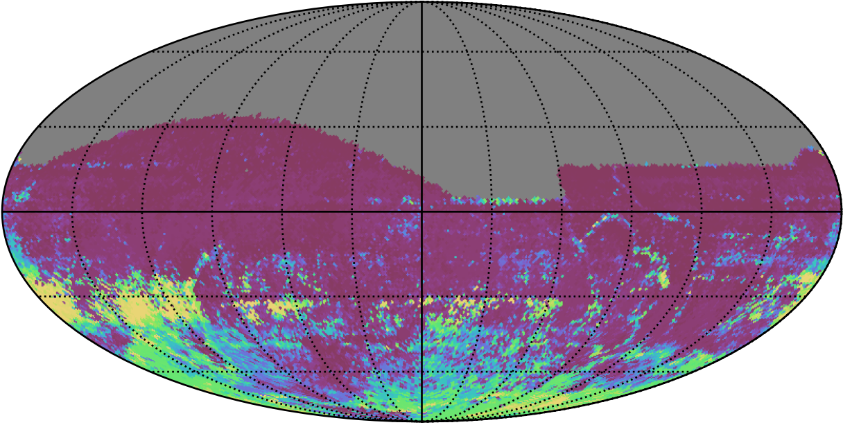
ddf_acor_sf15_ls40_lsr50_v3.4_10yrs All sky r band: 75th Percentile Intranight Timespan
