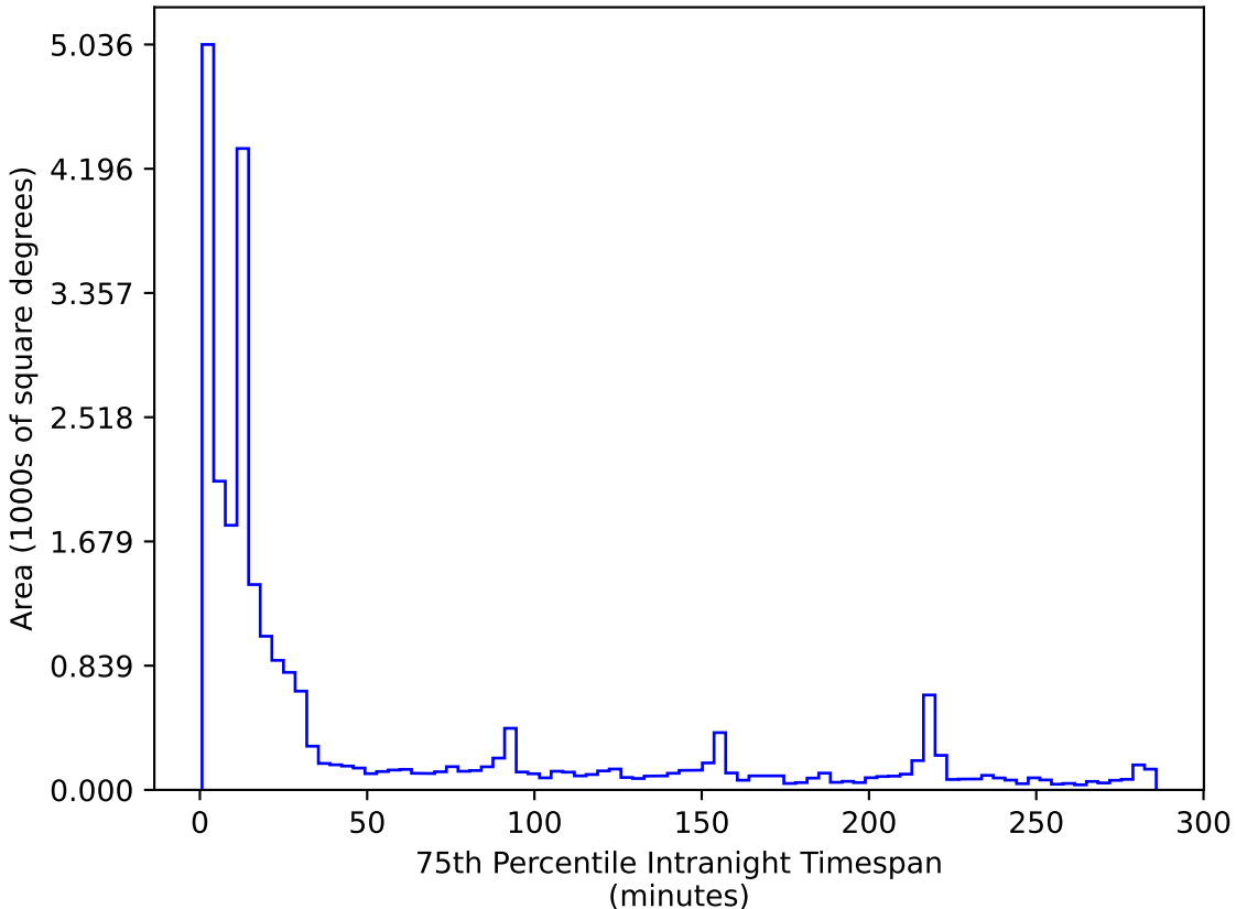
ddf_acor_sf15_lsf40_lsr50_v3.4_10yrs All sky r band: 75th Percentile Intranight Timespan
