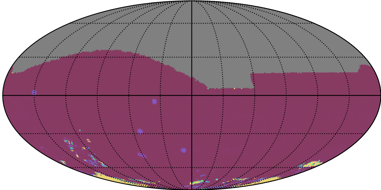
ddf_acor_sf15_lsf40_lsr50_v3.4_10yrs All sky iz bands: 75th Percentile Intranight Timespan
