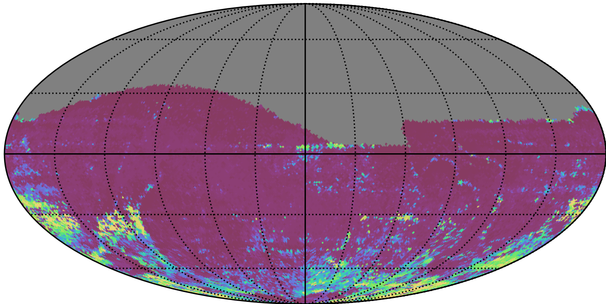
ddf_acor_sf15_lsf40_lsr50_v3.4_10yrs All sky i band: 75th Percentile Intranight Timespan
