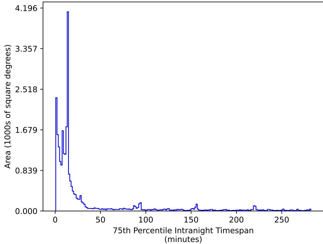
ddf_acor_sf15_lsf40_lsr50_v3.4_10yrs All sky i band: 75th Percentile Intranight Timespan
